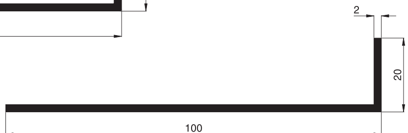
10 91 40 Winkelprofil 100/20/2
