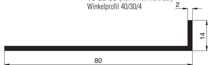
10 91 28 Winkelprofil 80/14/2
