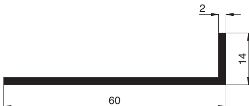
10 91 08 Winkelprofil 60/14/2
